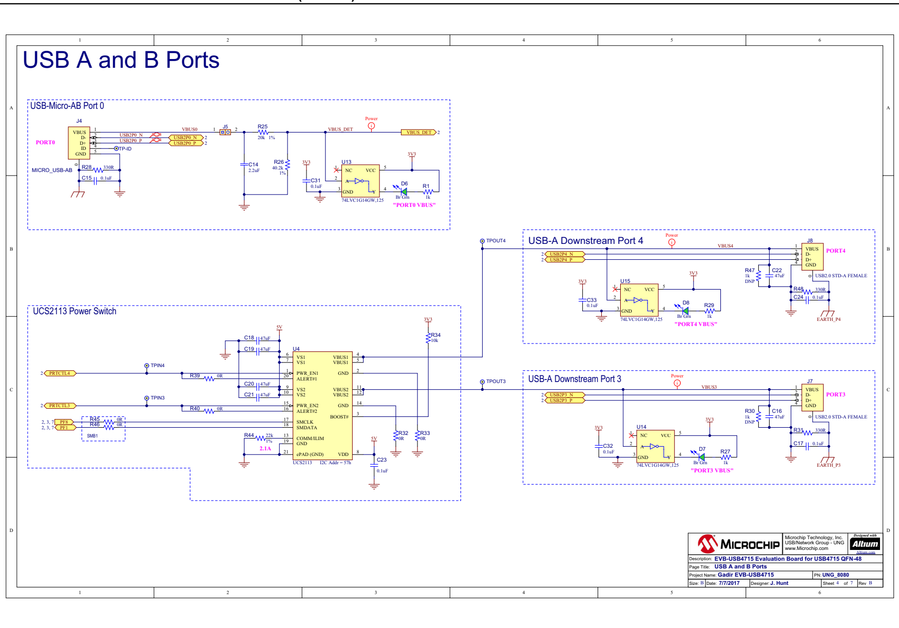
FIGURE A-4: EVB-USB4715 SCHEMATIC (PAGE 4)
