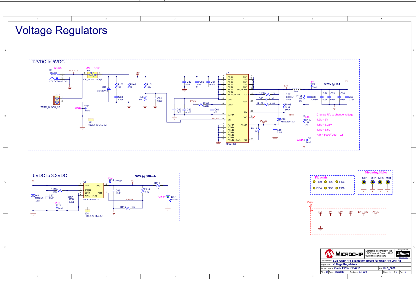
FIGURE A-6: EVB-USB4715 SCHEMATIC (PAGE 6)
