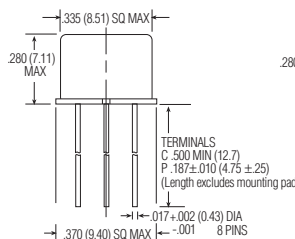
MGA/MGAD/MGADD ENCLOSURE
