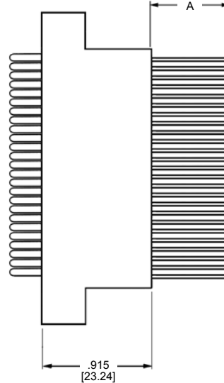
Plug Assembly
