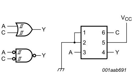
Fig 8. 2-input OR gate or 2-input NAND gate with both inputs inverted
