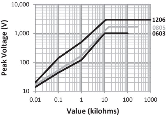
1.2/50µs Pulse Performance
