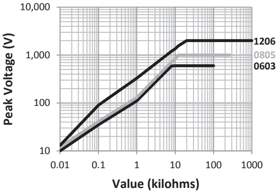
10/700µs Pulse Performance
