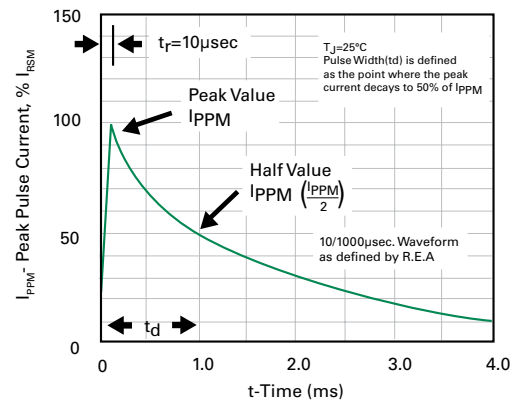
Figure 4 - Test Pulse Waveform
