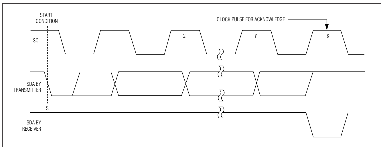
Figure 6. Acknowledge
