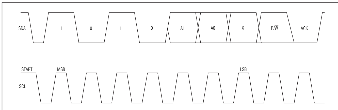
Figure 7. Slave Address
