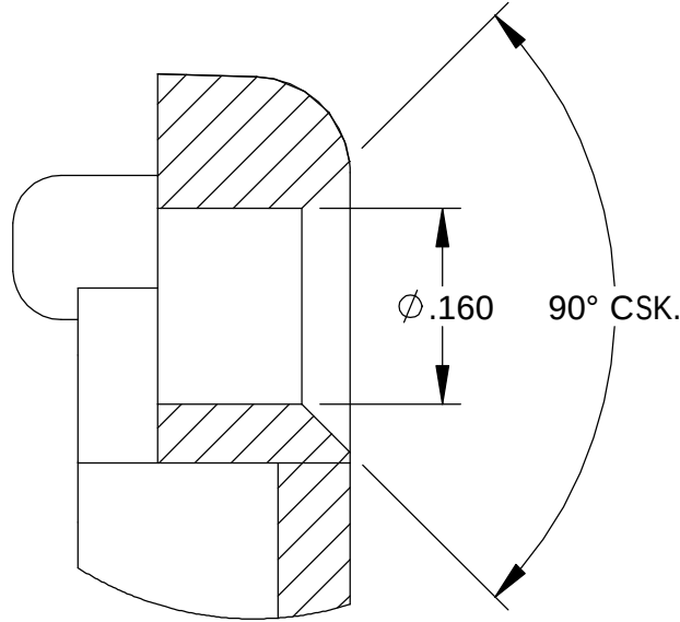
DETAIL D SCALE 6 : 1
