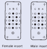
Female insert
