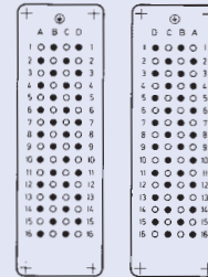
Female insert
