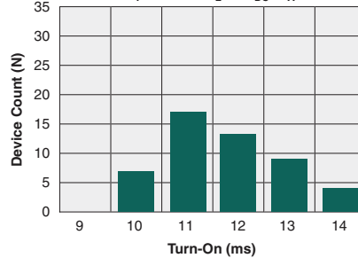
Typical Turn-On Time ( N=50 , I_F=20\text{mA} , I_L=1A_{DC} , T_A=25^\circ\text{C} )
