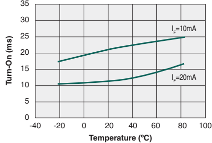
Typical Turn-On vs. Temperature ( I_L=1A_{DC} )
