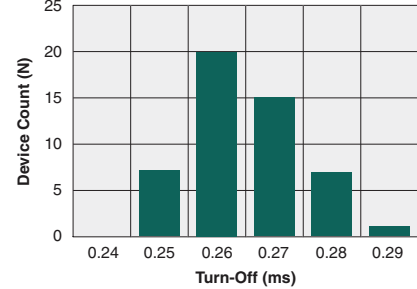
Typical Turn-Off Time ( N=50 , I_F=20\text{mA} , I_L=1A_{DC} , T_A=25^\circ\text{C} )
