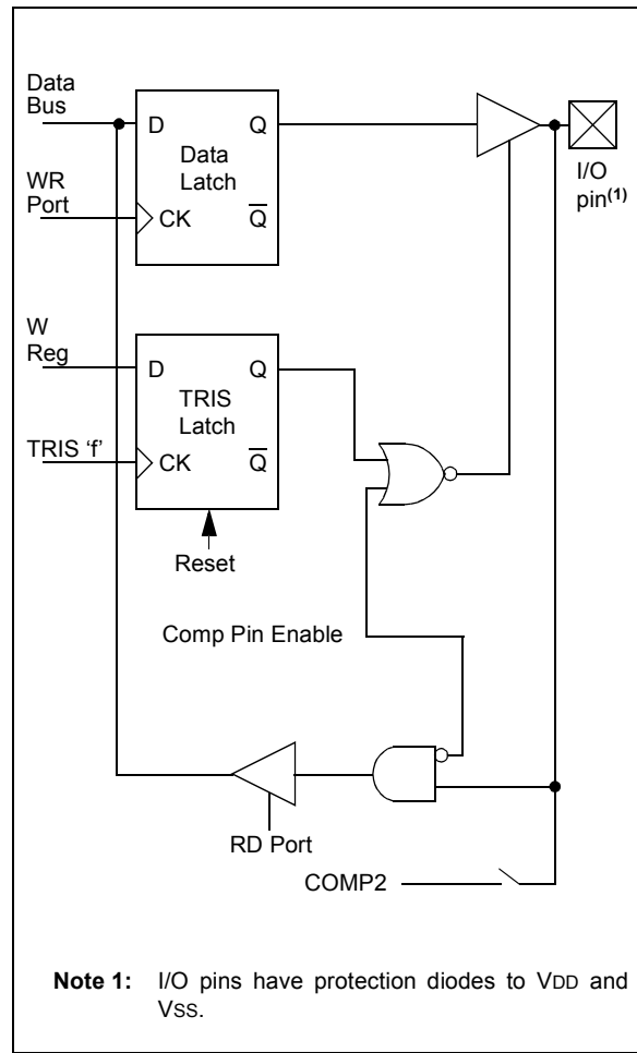
FIGURE 5-9: BLOCK DIAGRAM OF RC0/RC1
