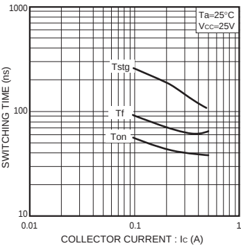
Fig.2 Switching Time
