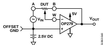
Figure 41. Inverting Programmable Gain
