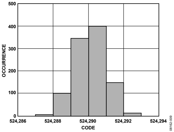
Figure 9. C Grade Noise Distribution Histogram ( V_{REF} = AV_{DD} , Update Rate = 16.7 Hz, Gain = 128)
