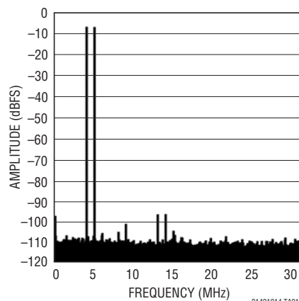
2-Tone FFT, f_{IN} = 70MHz and 69MHz
