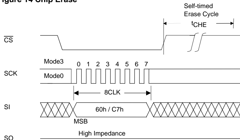
Figure 14 Chip Erase
