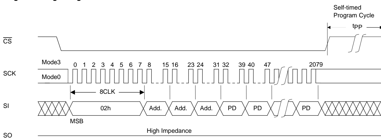
Figure 15 Page Program
