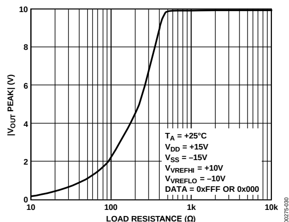
Figure 29. Output Swing vs. Load Resistance
