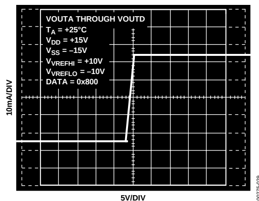
Figure 28. DAC Output Current vs. V_{OUTx}
