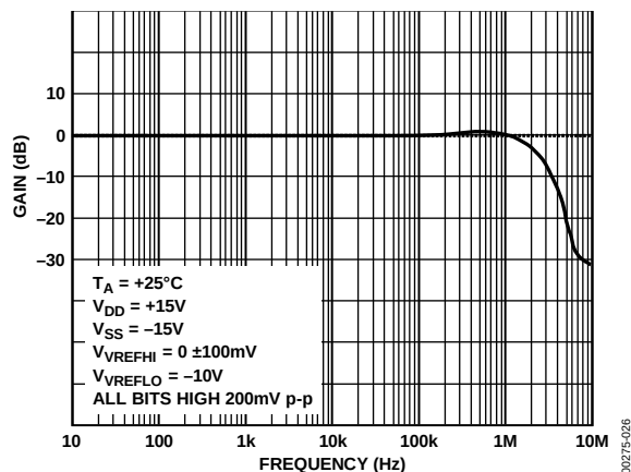
Figure 25. Small-Signal Response
