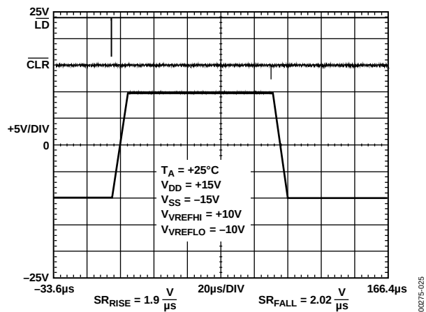
Figure 24. Slew Rate ( \pm 15 \text{ V} )
