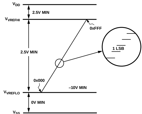
Figure 30. Output Voltage Range Programming
