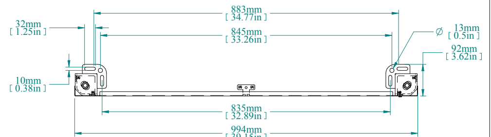
TOP VIEW
