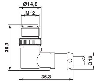
Dimensioned drawing
