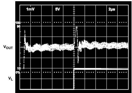
Figure 28. Load Crosstalk
