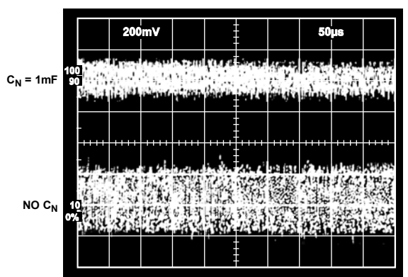
Figure 8. Effect of 1\text{ }\mu\text{F} Noise Reduction Capacitor on Broadband Noise
