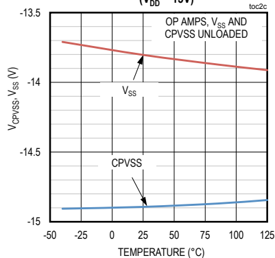
CPVSS AND V_{SS} vs. TEMPERATURE ( V_{DD} = 15V )
