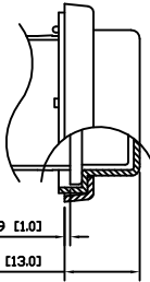
ASSEMBLED VIEW
