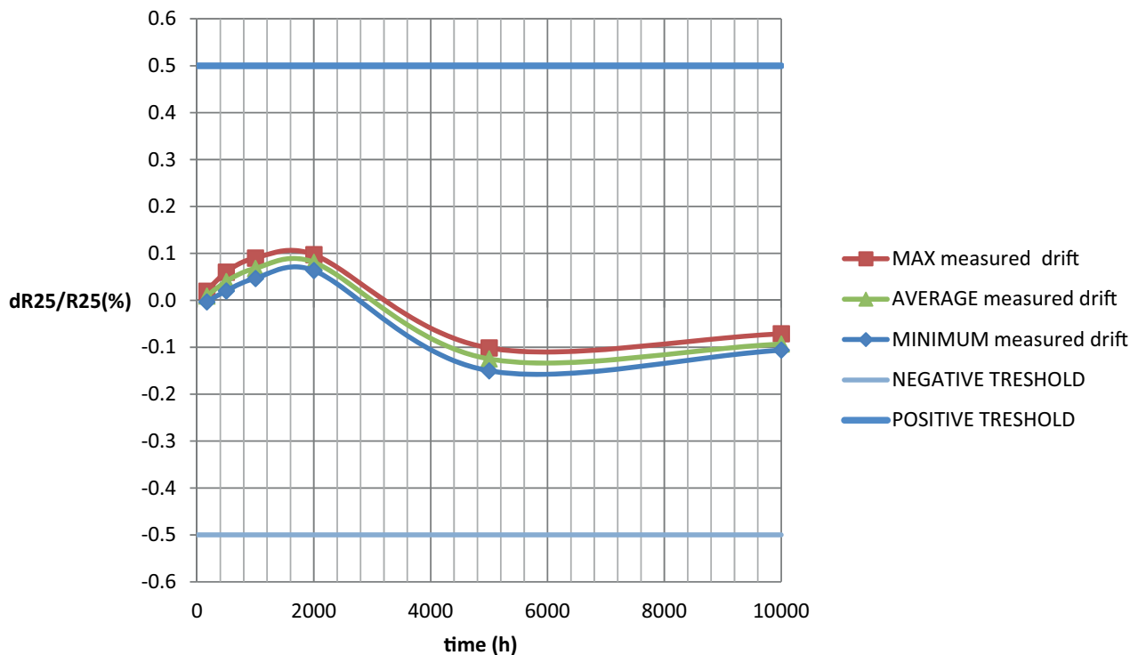
Fig. 1 - R_{25}^{\circ C} Drift after Storage at 125 °C for 0603 Case
