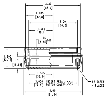
VIEW A-A SCALE 1:1
