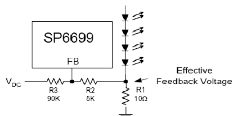
Fig. 24: Dimming Control using a DC Voltage
