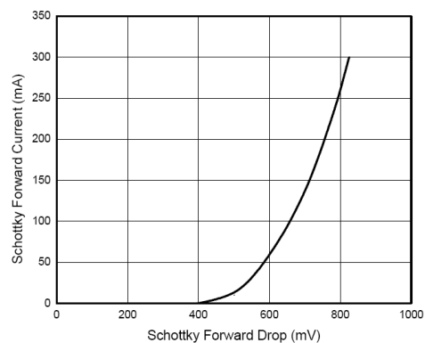
Fig. 7: Schottky Forward Current vs Schottky Forward Drop
