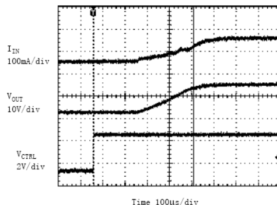
Fig. 20: Soft Start Waveform V_{\text{IN}} = 3.6\text{V} , 4 LEDs, I_{\text{LED}} = 20\text{mA}
