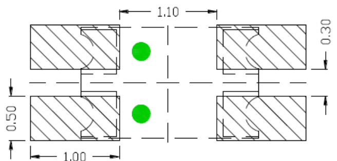
Figure 1. IN-S85TATRGB Solder Pattern
