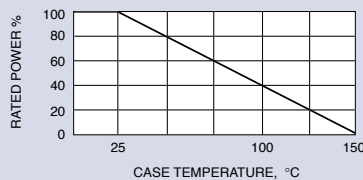
Derating Curve
