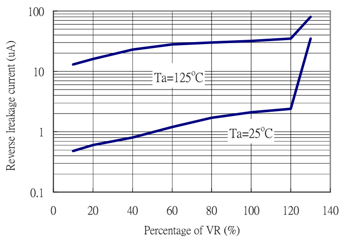
FIG 4 Maximum reverse leakage character
