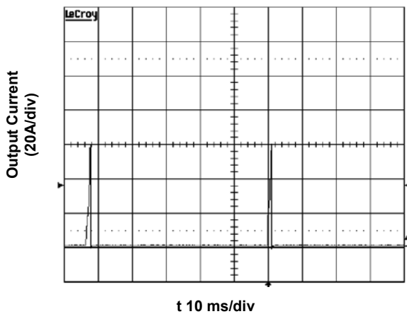
Figure 10. Short Circuit Current. Vin = 24V
