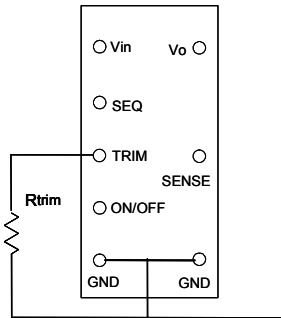
Figure 16. Circuit to Trim Output Voltage
