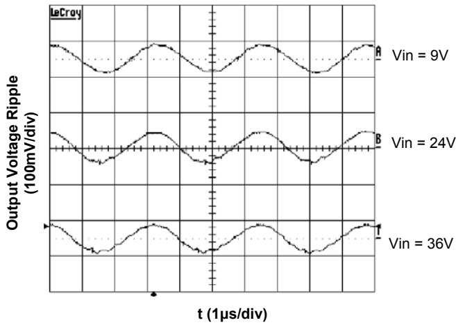
Figure 6. Output Ripple Voltage at 5V, 9A Output
