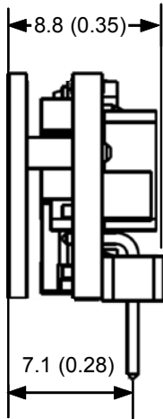
Side View with Baseplate
