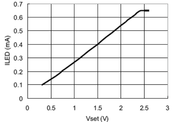
12. I_{LED} VS V_{SET} ( V_{IN}=16\text{V} , 3 LEDs, 100\mu\text{H} , R_s=0.3\Omega )
