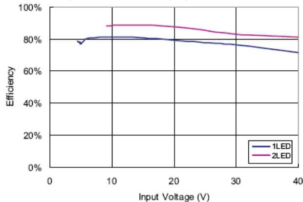
3. Efficiency vs Input Voltage ( R_s = 0.067\Omega , L = 47\mu\text{H} )
