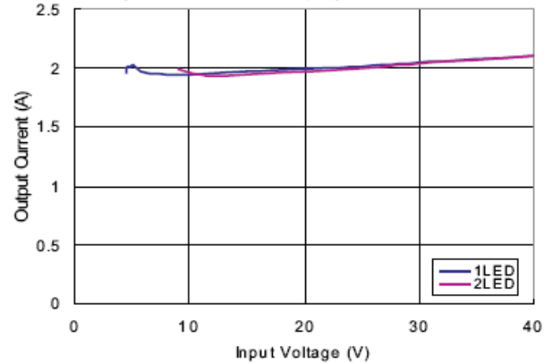
4. Output Current vs Input Voltage ( R_s = 0.067\Omega , L = 47\mu\text{H} )
