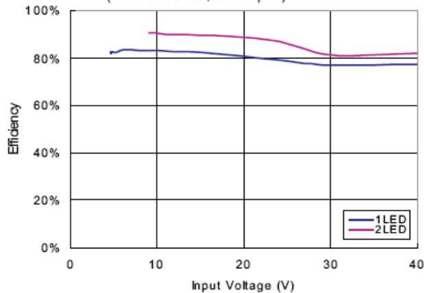
3. Efficiency vs Input Voltage ( R_s = 0.067\Omega , L = 47\mu\text{H} )
