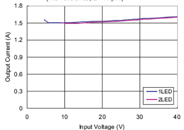
6. Output Current vs Input Voltage ( R_s = 0.1\Omega , L = 47\mu\text{H} )
