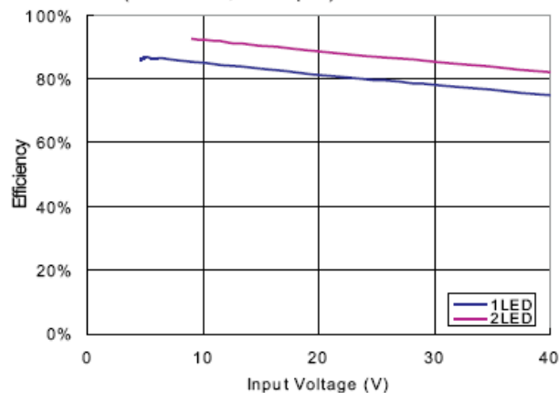
5. Efficiency vs Input Voltage ( R_s = 0.1\Omega , L = 47\mu\text{H} )
