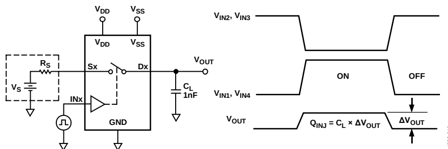
Figure 19. Charge Injection
