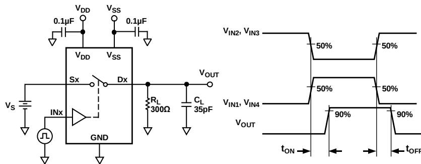
Figure 17. Switching Times
