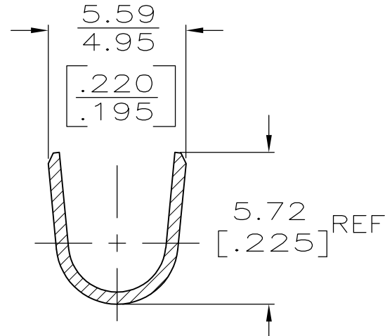
SECTION C-C
