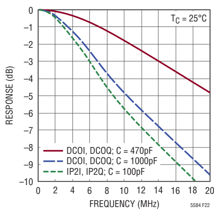
Figure 22. Input Response Bandwidth for the DCOI, DCOQ, IP2I and IP2Q Pins
