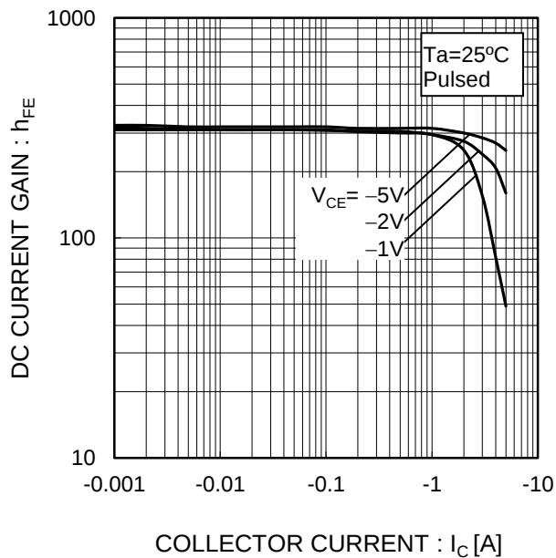
Fig.4 DC Current Gain vs. Collector Current(I)
