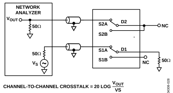
Figure 28. Channel-to-Channel Crosstalk (S1A-S2A)
