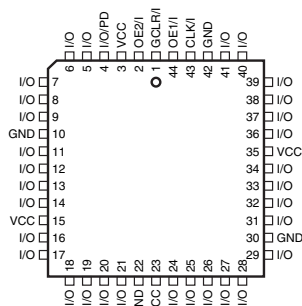
PLCC Top View
