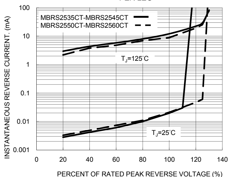
FIG. 5 TYPICAL REVERSE CHARACTERISTICS PER LEG
