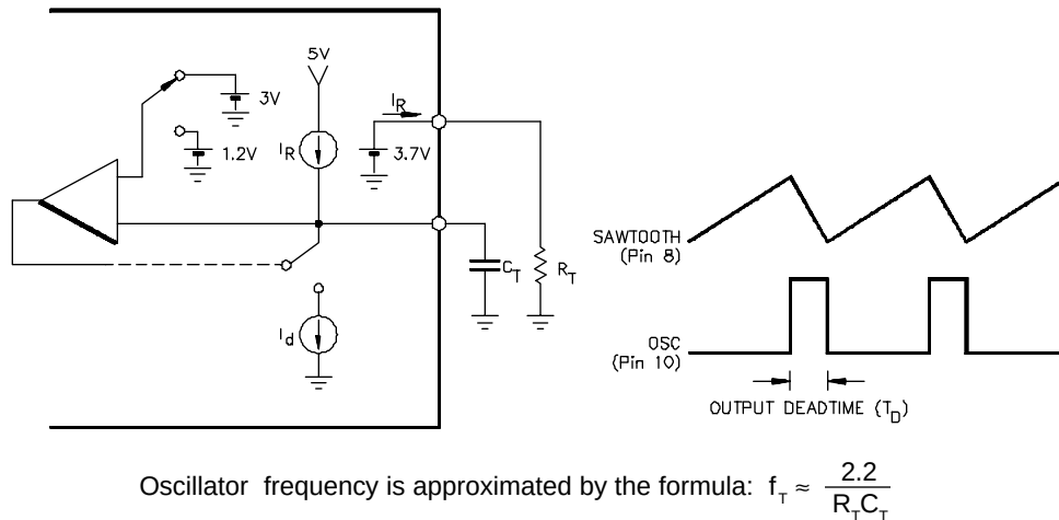
FIGURE 20 - OSCILLATOR CIRCUIT
