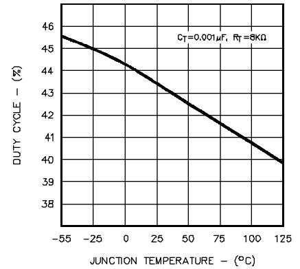
FIGURE 18. DUTY CYCLE VS. TEMPERATURE
