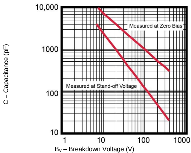
FIGURE 4 Typical Capacitance vs. Breakdown Voltage (unidirectional configuration) NOTE: Bidirectional capacitance is half that shown at zero volts.
