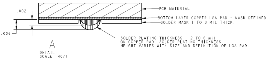
BOTTOM SURFACE OF PCB
