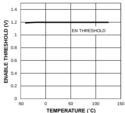
EN Threshold vs. Temperature
