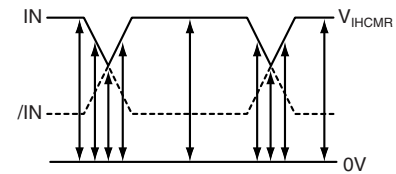
Figure 5a. Input Common Mode, PECL, LVPECL
