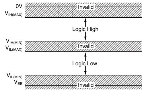
Figure 4c. Input Levels, NECL
