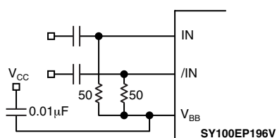
Figure 8. Re-Biasing an AC-Coupled Signal
