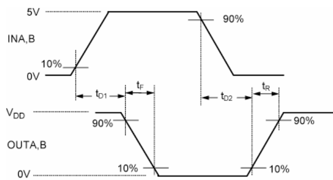
Inverting Driver
