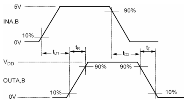
Non-Inverting Driver
