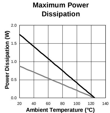
Figure 5c. Maximum P_{DISS} vs. Ambient Temperature
