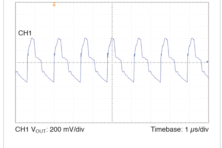
Figure 16 — Output voltage ripple, V_{IN} = 28\text{ V} , V_{OUT} = 24.0\text{ V} , C_{OUT\_EXT} = 250\text{ }\mu\text{F} , R_{LOAD} = 1.791\text{ }\Omega
