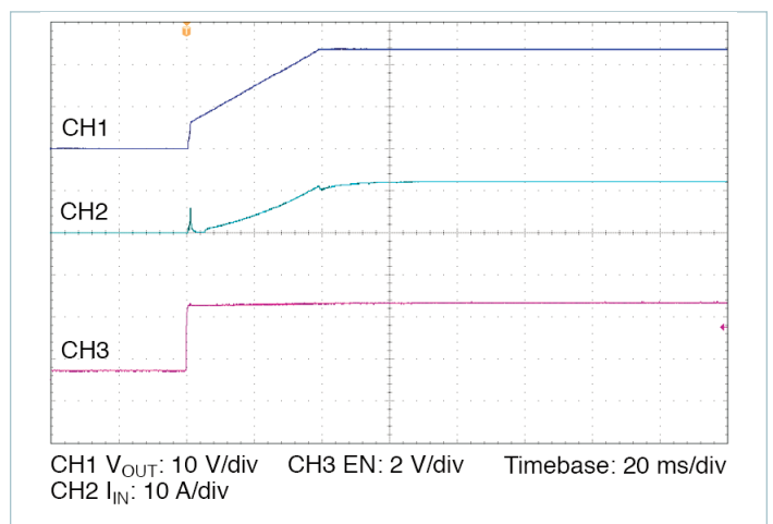
Figure 14 — Startup from EN, V_{IN} = 28\text{ V} , C_{OUT\_EXT} = 2500\text{ }\mu\text{F} , R_{LOAD} = 1.791\text{ }\Omega
