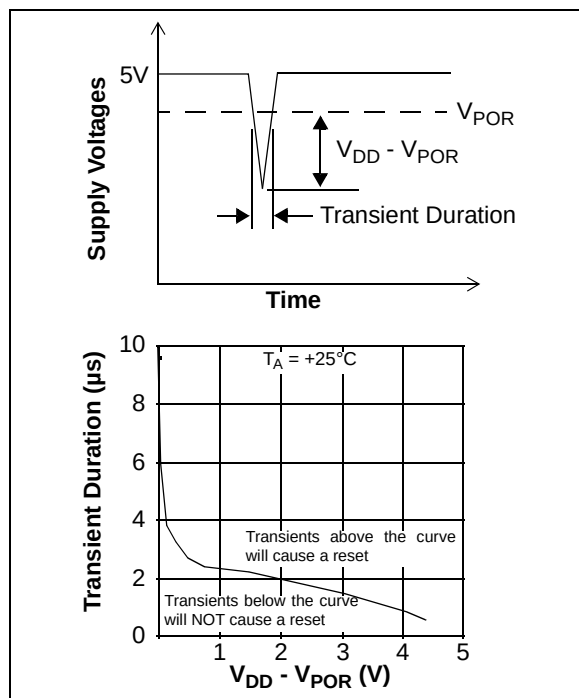
FIGURE 4-3: Typical Transient Response.
