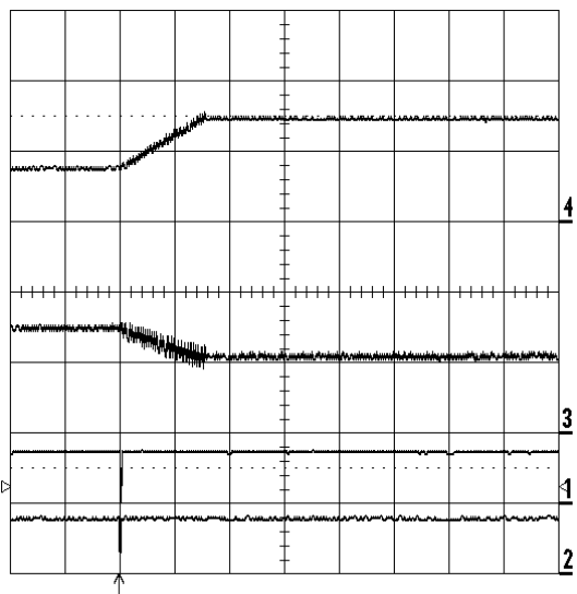
Waveform when it drives from code 511 to code 256
