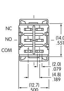
Double Pole
